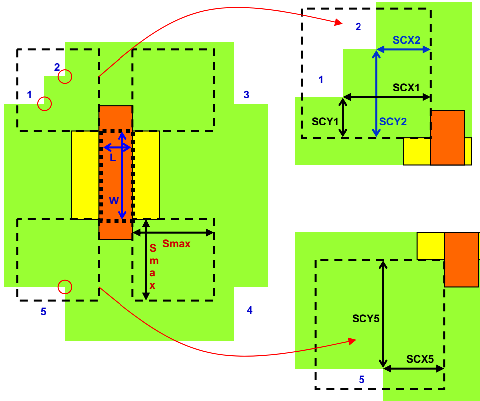
Equation 7 Closed form solution to corners_C equation
